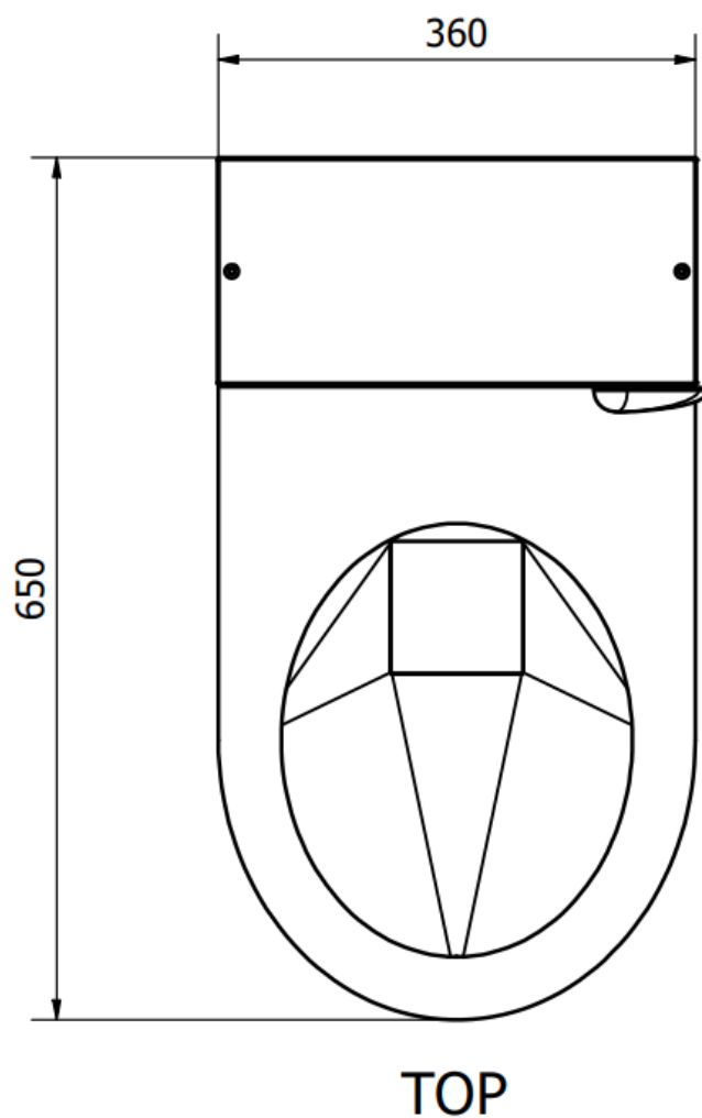
TOP VIEW · B17656(CTP) top view; dimensions in millimetres.
