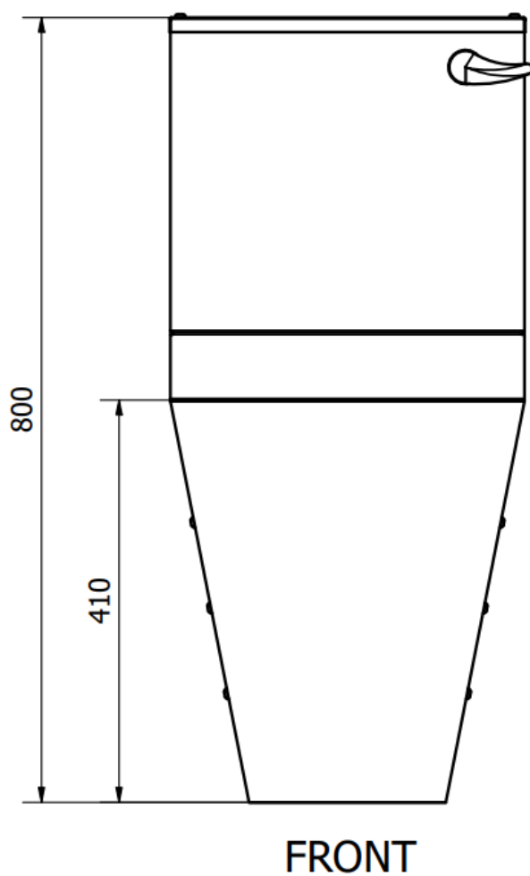
FRONT VIEW · B17656(CTP) front view; dimensions in millimetres.
