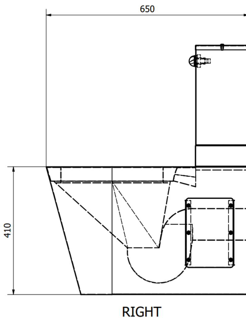
RIGHT VIEW · B17656(CTP) right-side view; dimensions in millimetres.
