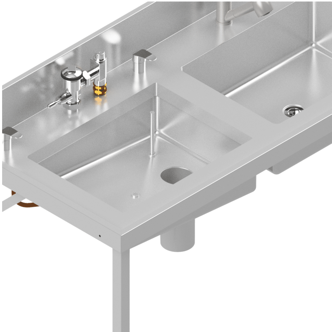
PRODUCT IMAGE · 1830 mm left-hand T3 configuration shown.
