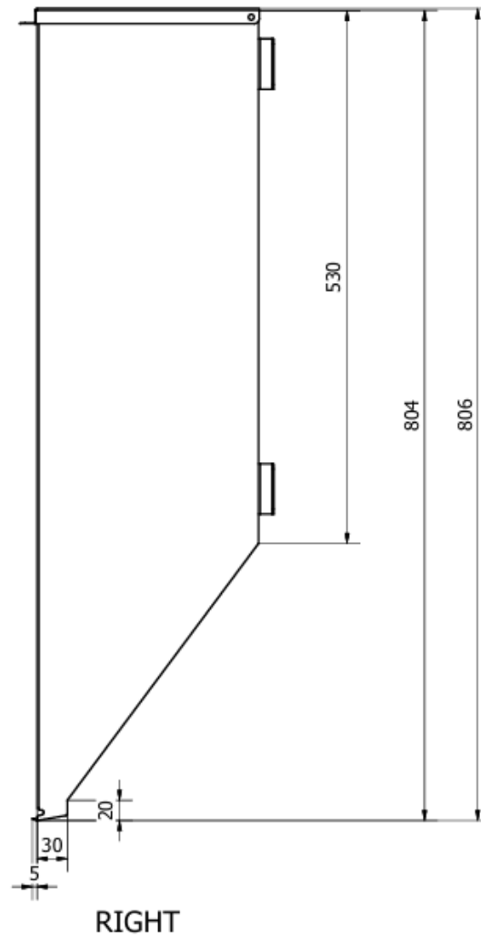
RIGHT VIEW · B30848 right view; dimensions in millimetres.
