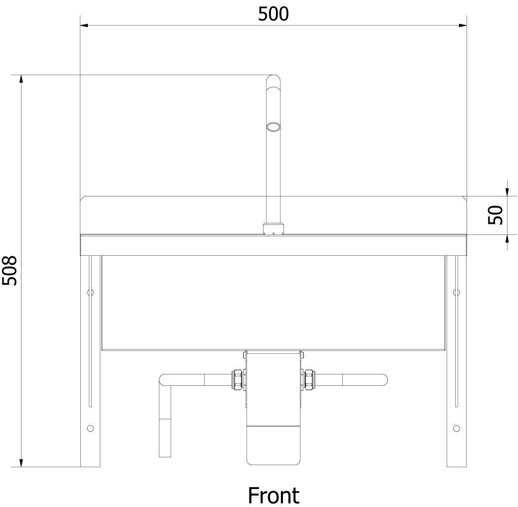
PRODUCT IMAGE · B36658(D) front view: demand model with 50mm standard splashback. Dimensions in mm. Model-specific reference; other configurations are not shown.
