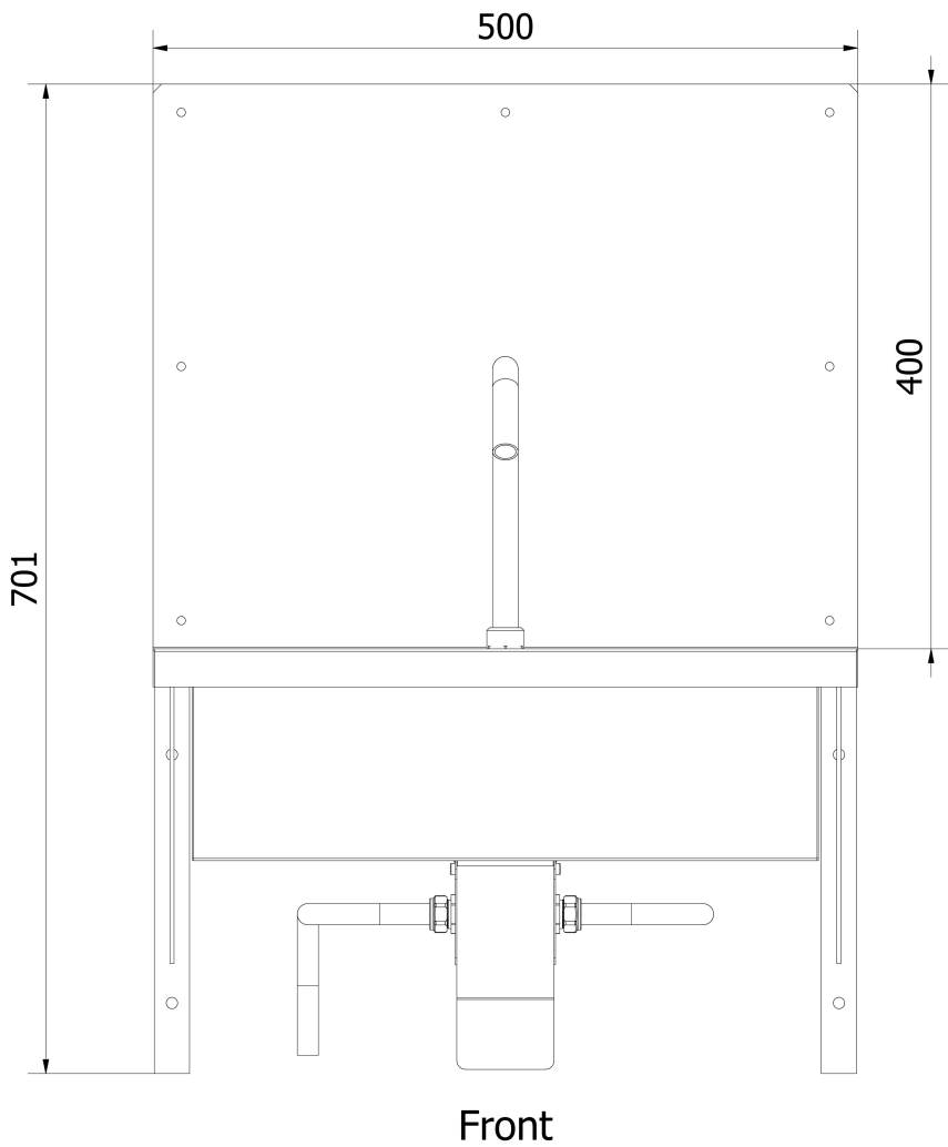
PRODUCT IMAGE · B36658(DE) front view: demand model with 400mm extended splashback. Dimensions in mm. Model-specific reference; other configurations are not shown.
