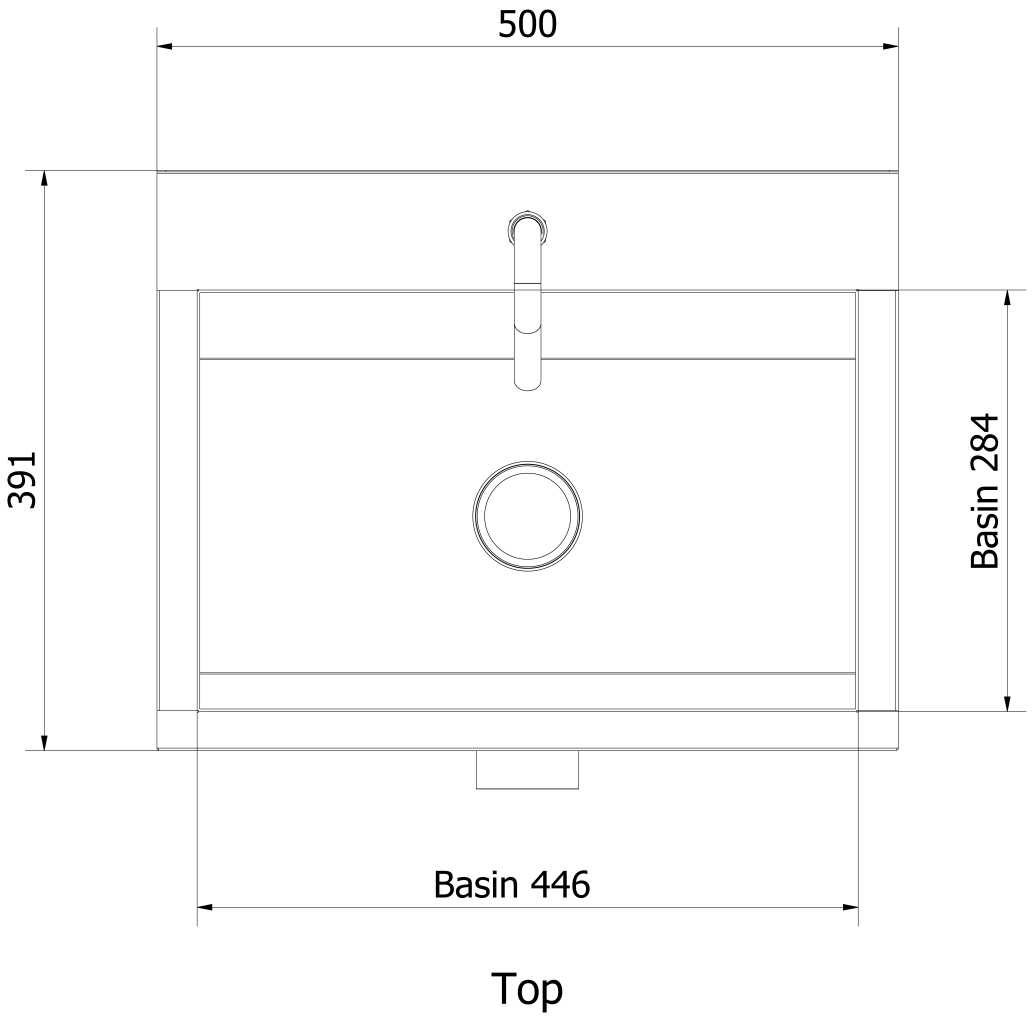
PRODUCT IMAGE · B36658(D) top view: demand model with 50mm standard splashback. Dimensions in mm. Model-specific reference; other configurations are not shown.
