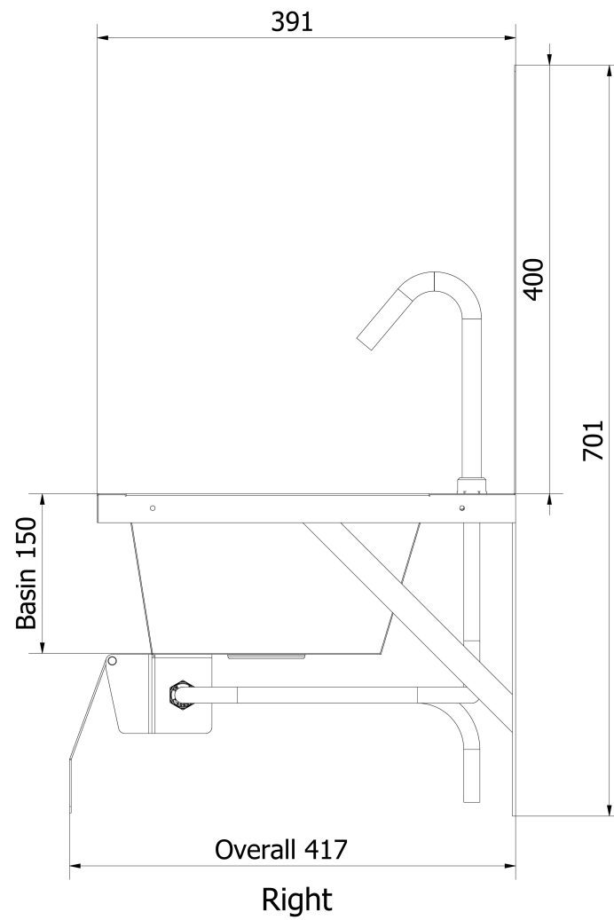
PRODUCT IMAGE · B36658(DE) right view: demand model with 400mm extended splashback. Dimensions in mm. Model-specific reference; other configurations are not shown.
