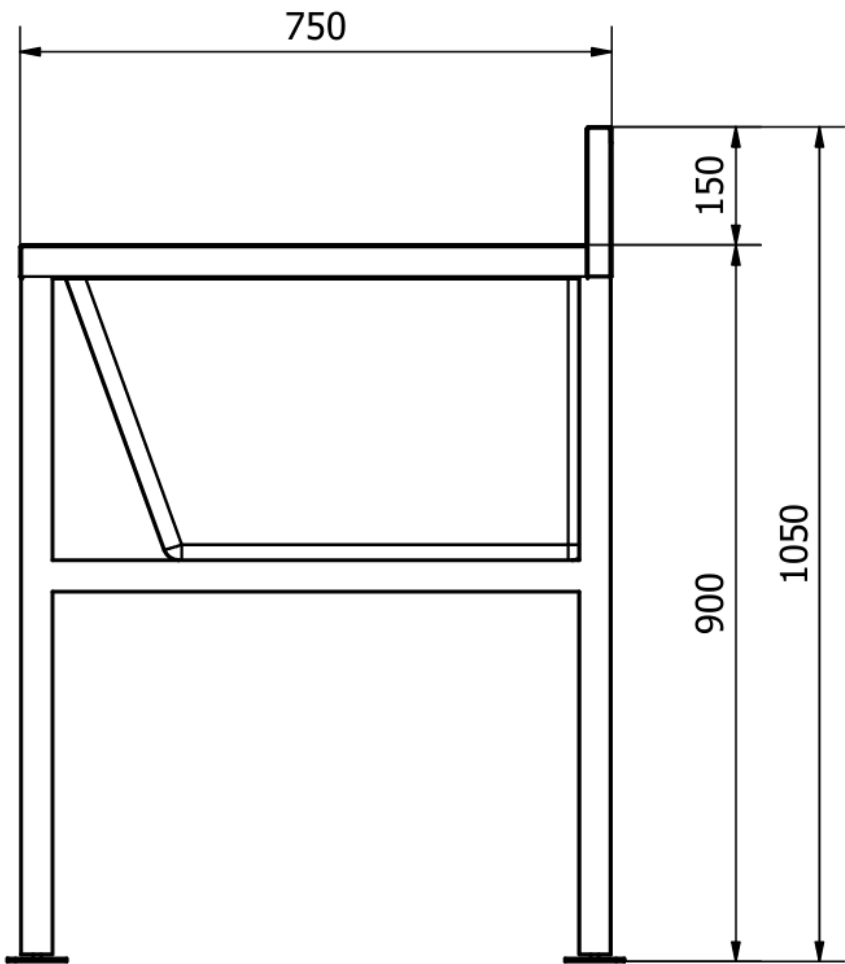
RIGHT
