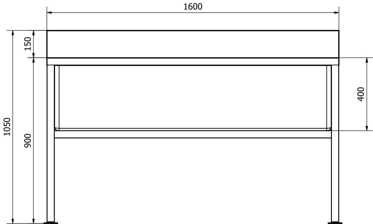
FRONT
