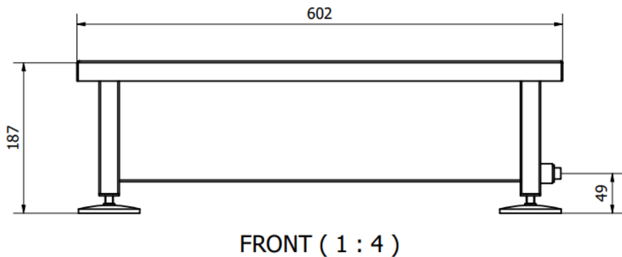
FRONT VIEW · Front view. Dimensions in mm; image reproduced to fit the page.
