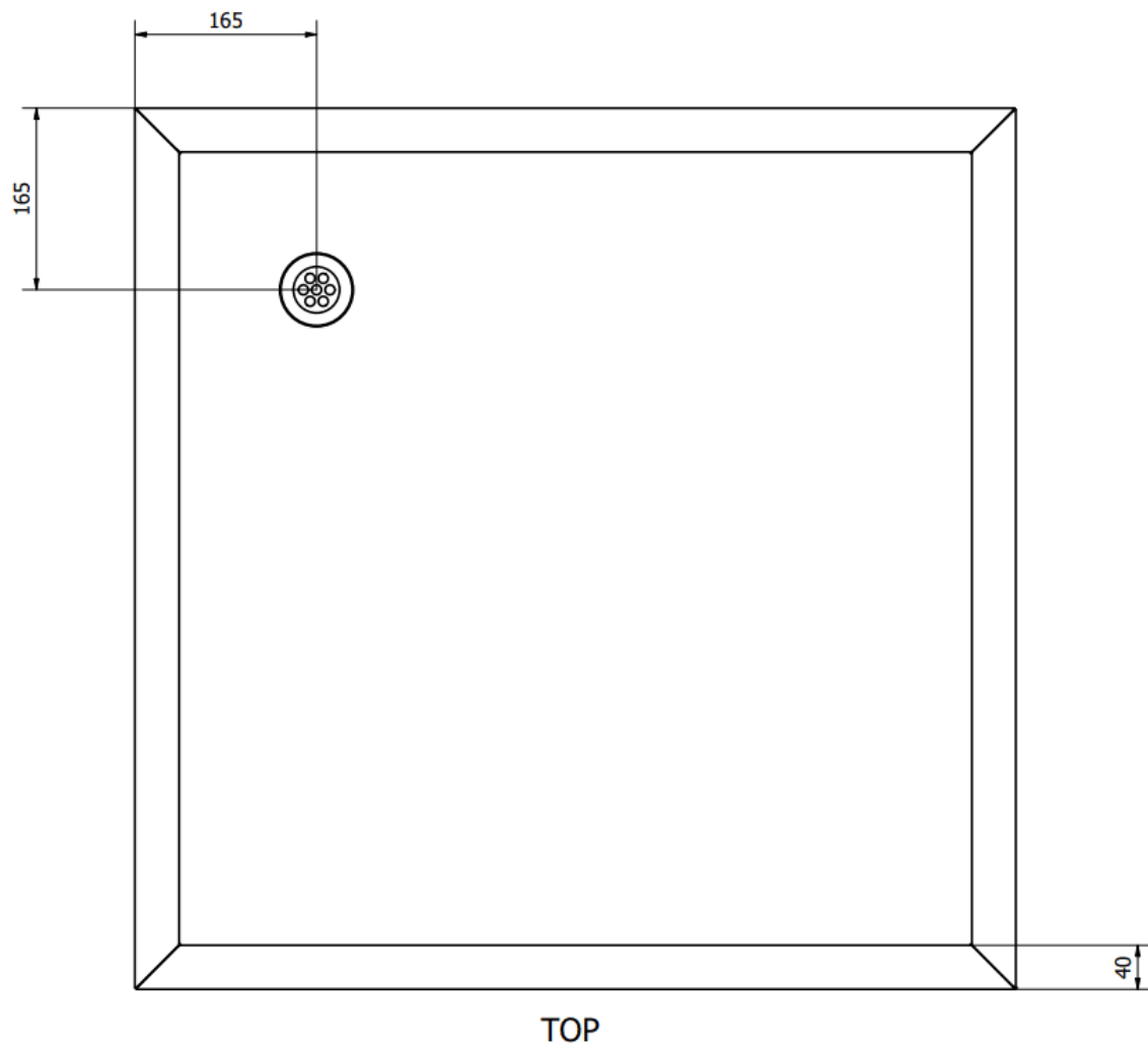
TOP VIEW · B75130 technical drawing – top view
