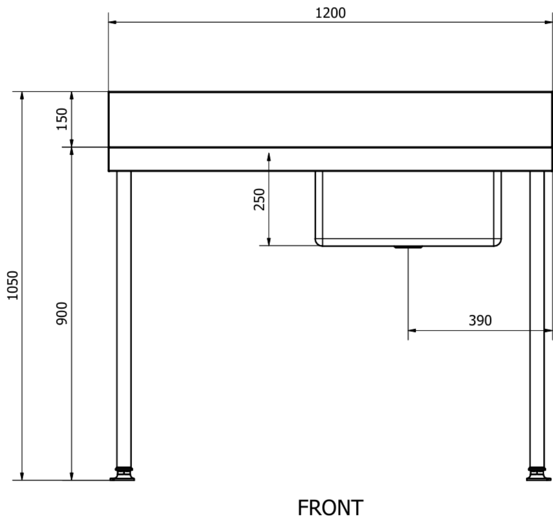
FRONT VIEW · 1200 mm model: 900 mm working height and 1050 mm overall height
