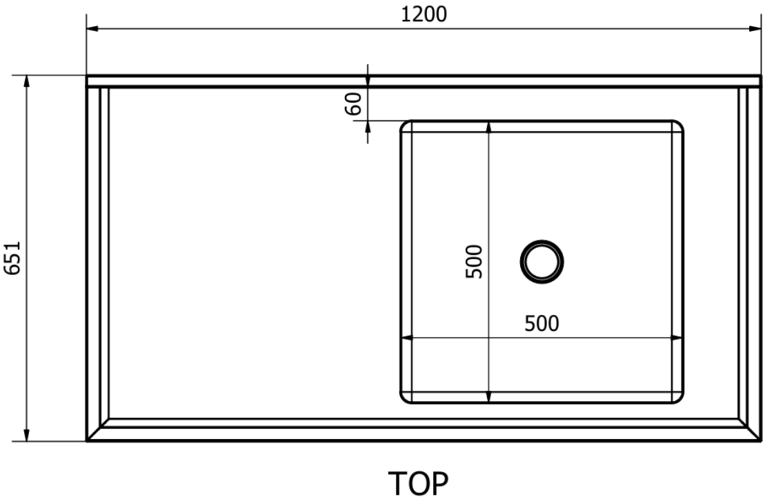
TOP VIEW · Top view: source drawing labels the width 651 mm; specified catalogue width is 650 mm
