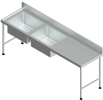
PRODUCT IMAGE · E22128(DL-112-2400): 2400 mm, 1.2 mm Grade 304, two 600 x 500 x 300 mm left-hand bowls
