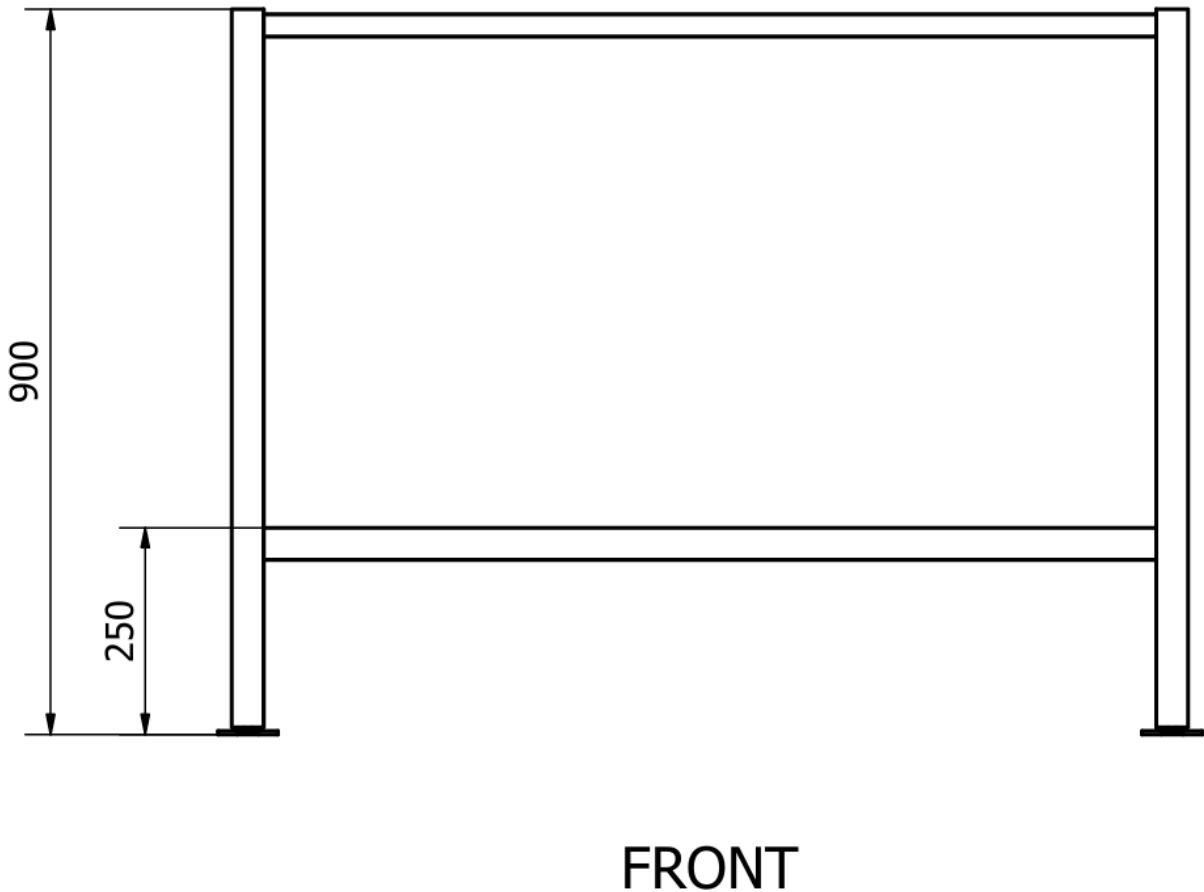
FRONT VIEW · Front view of the 1200mm x 750mm pot drying rack; overall height 900mm. Dimensions in millimetres.
