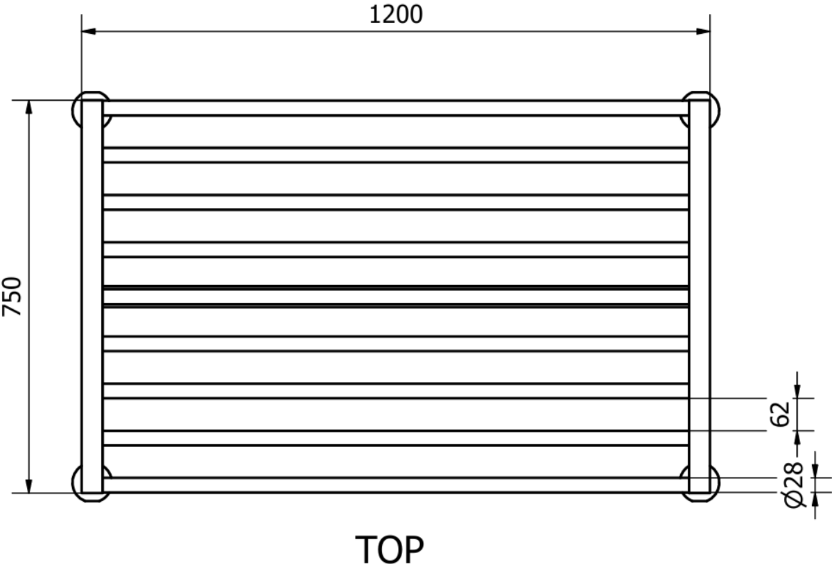
TOP VIEW · Top view showing the 1200mm overall length, 750mm overall width and \varnothing 28 mm round tube cross members. Dimensions in millimetres.
