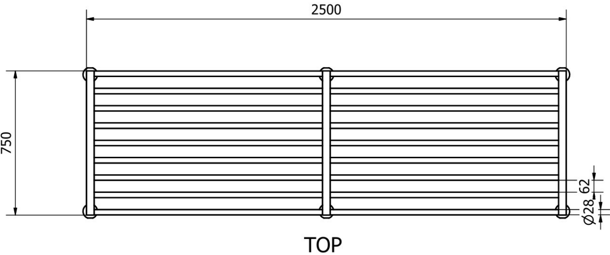
TOP VIEW · Overall length 2500mm and width 750mm; centre supports and Ø28mm round tube cross members. Dimensions in millimetres.
