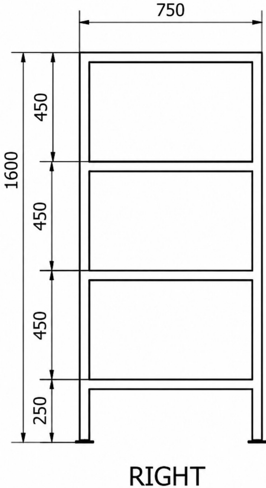
RIGHT VIEW · Overall width 750mm and height 1600mm, with 450mm tier pitch and lower frame at 250mm above the floor. Dimensions in millimetres.
